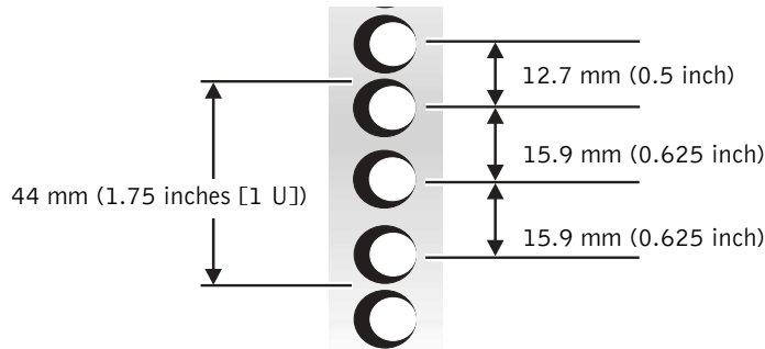
Figure 1-13. Two-Post, Open-Frame Relay Rack Universal-Hole Spacing
