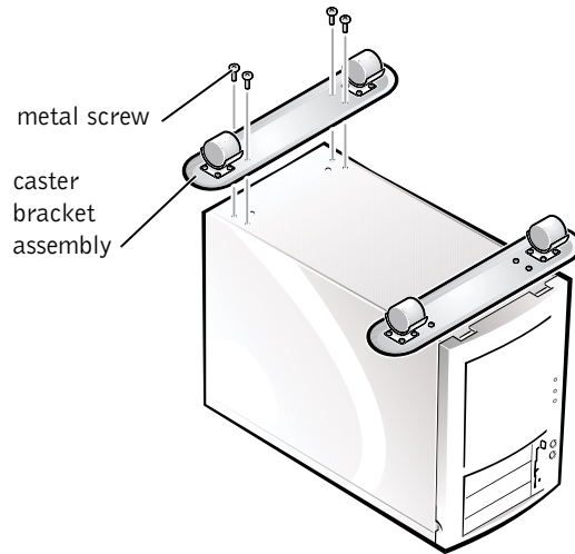
Figure 1-2. Attaching the Casters
