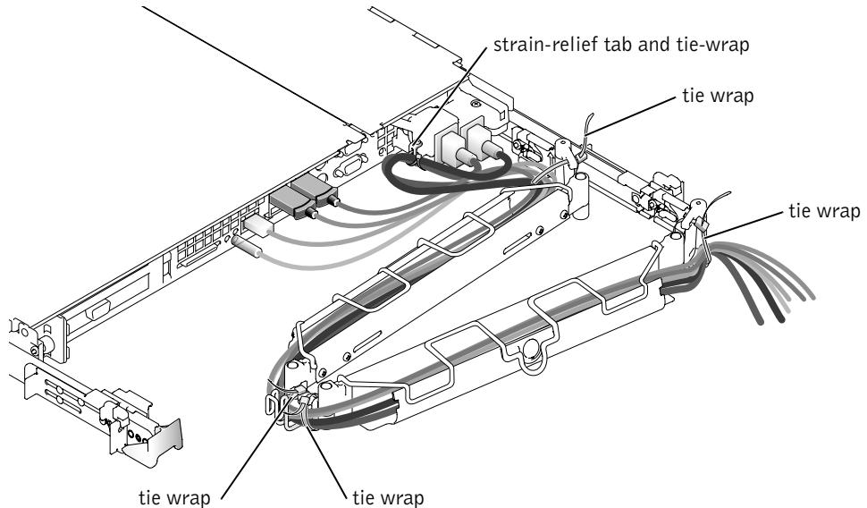
Figure 1-11. Routing Cables
