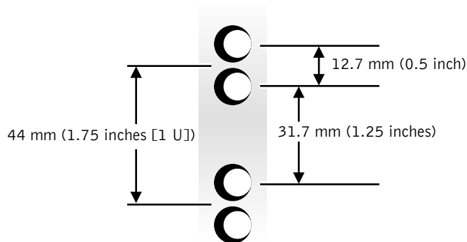
Figure 1-14. Two-Post, Open-Frame Relay Rack Wide-Hole Spacing
