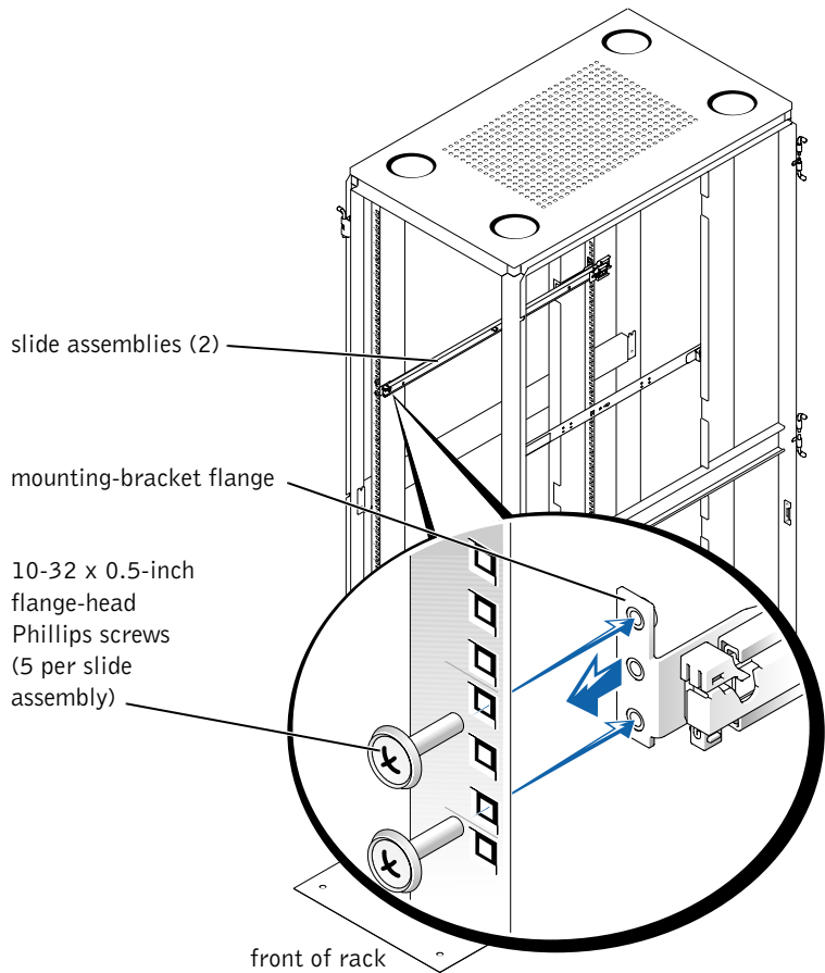
Figure 1-6. Installing the VersaRails Slide Assemblies
