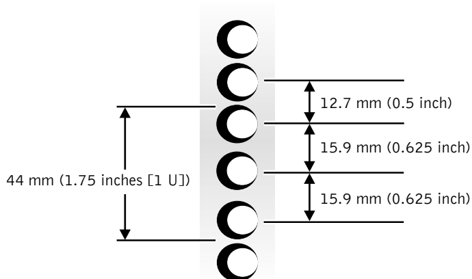
Figure 1-13. Two-Post, Open-Frame Relay Rack Universal-Hole Spacing
