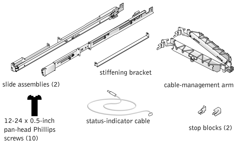
Figure 1-12. Two-Post Rack Kit Components
