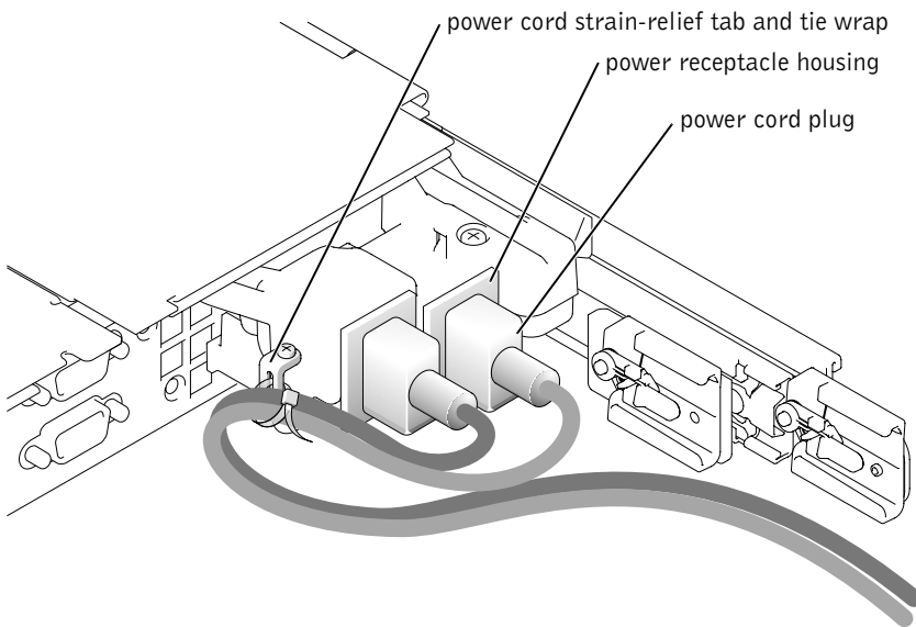
Figure 1-10. Installing the Power Cord Strain Relief
