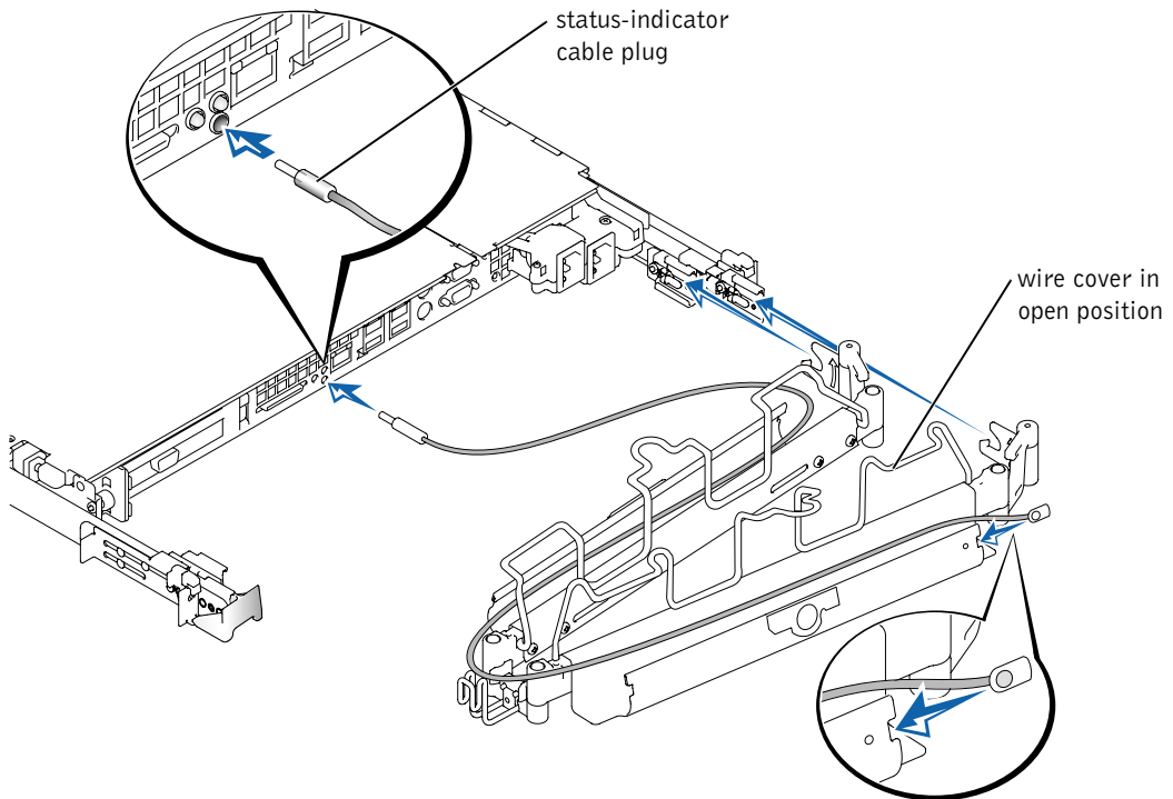
Figure 1-9. Opening the Wire Covers
