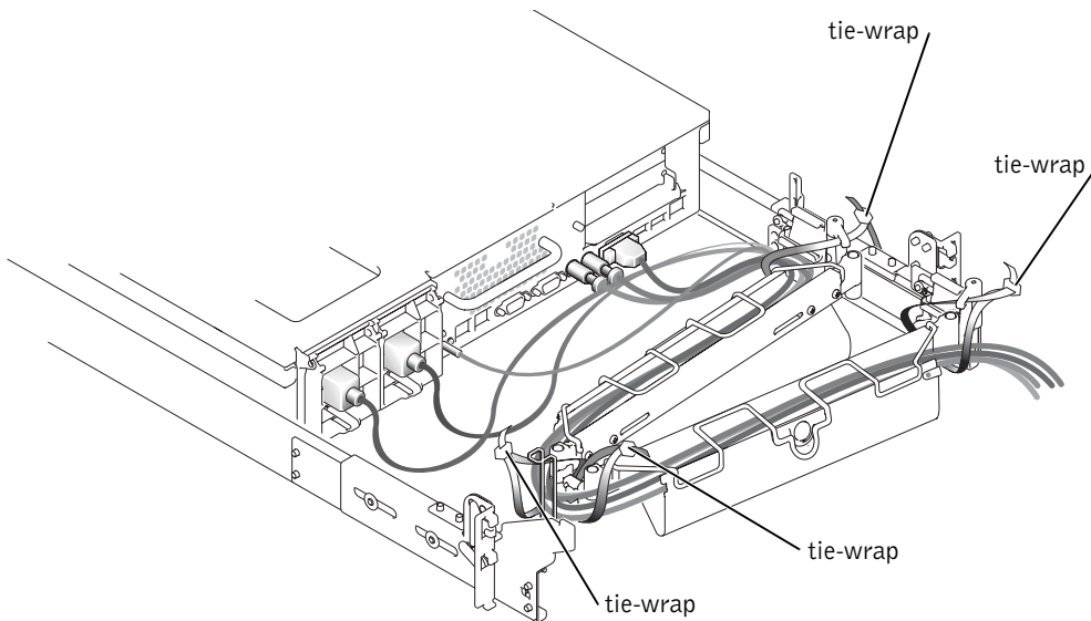
Figure 1-11. Routing Cables
