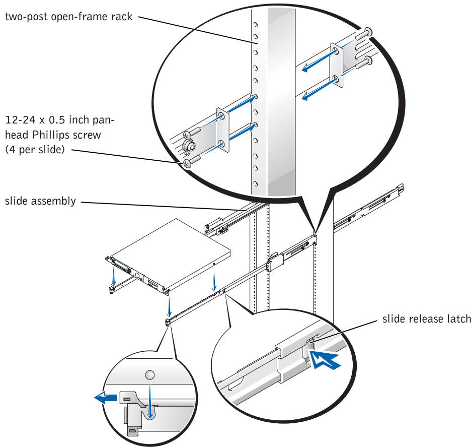
Figure 1-14. Installing the Slide Assemblies for Center-Mount Configuration
