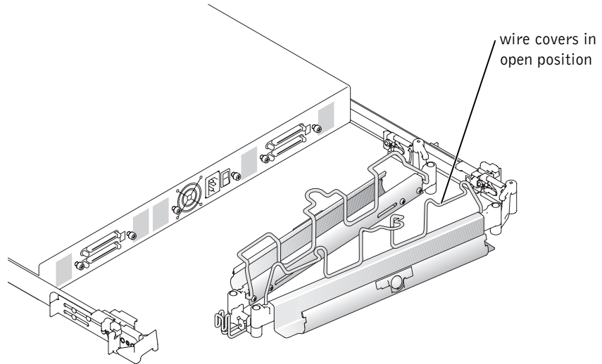
Figure 1-9. Opening the Wire Covers
