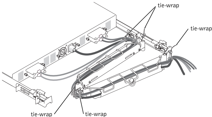
Figure 1-10. Routing Cables
