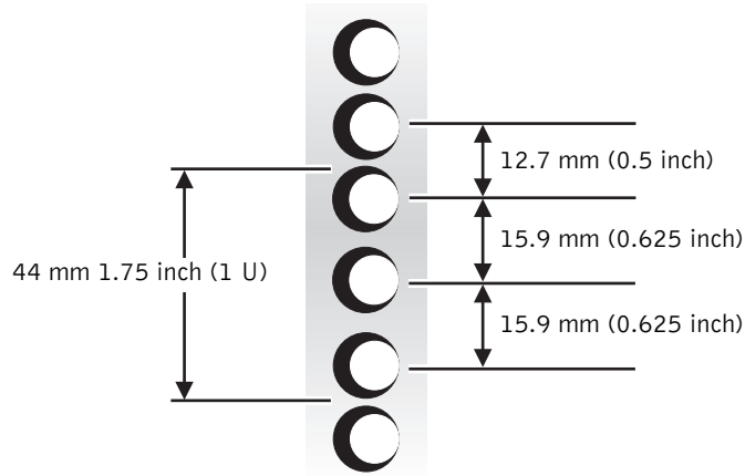
Figure 1-12. Two-Post, Open-Frame Relay Rack Universal-Hole Spacing
