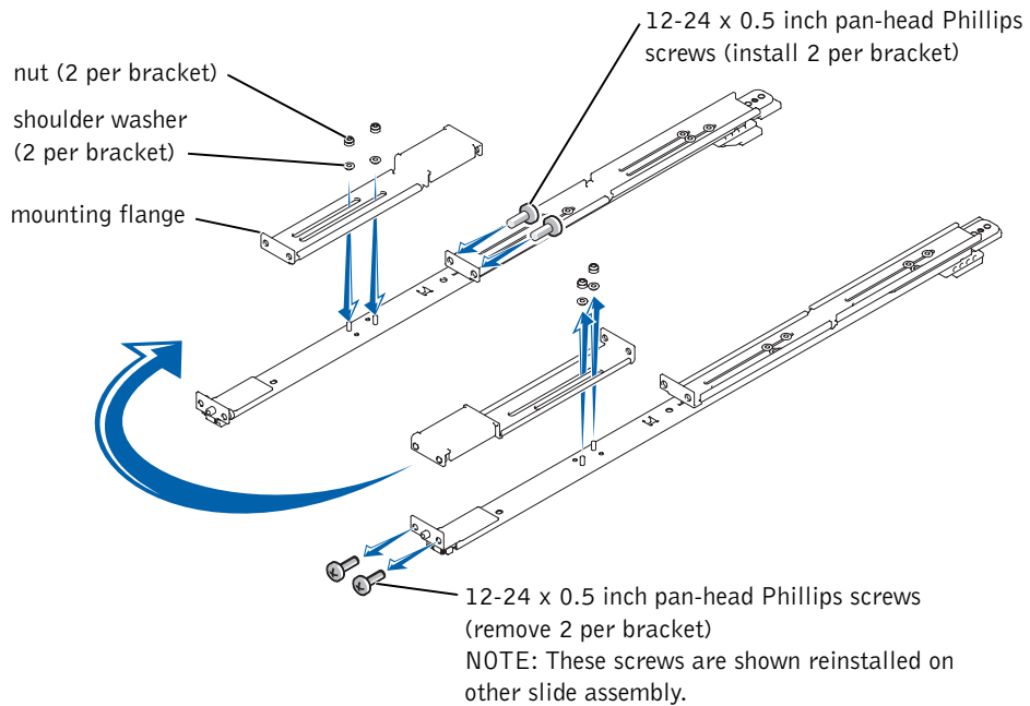
Figure 1-15. Rotating the Front Mounting Bracket for Flush-Mount Installation
