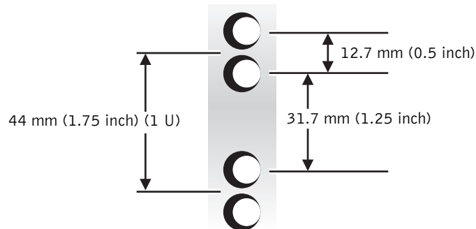
Figure 1-13. Two-Post, Open-Frame Relay Rack Wide-Hole Spacing
