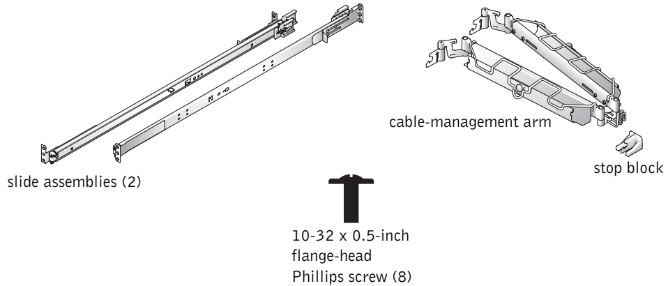
Figure 1-2. VersaRails Rack Kit Contents
