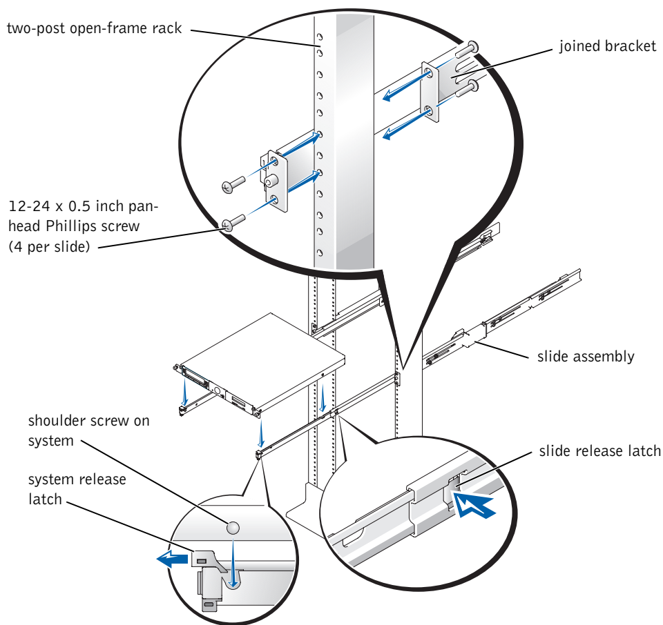
Figure 1-16. Installing the Slide Assemblies for Flush-Mount Configuration
