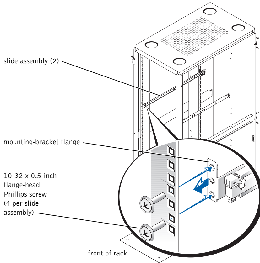
Figure 1-6. Installing the VersaRails Slide Assemblies
