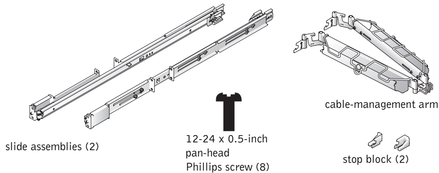
Figure 1-11. Two-Post Rack Kit Components
