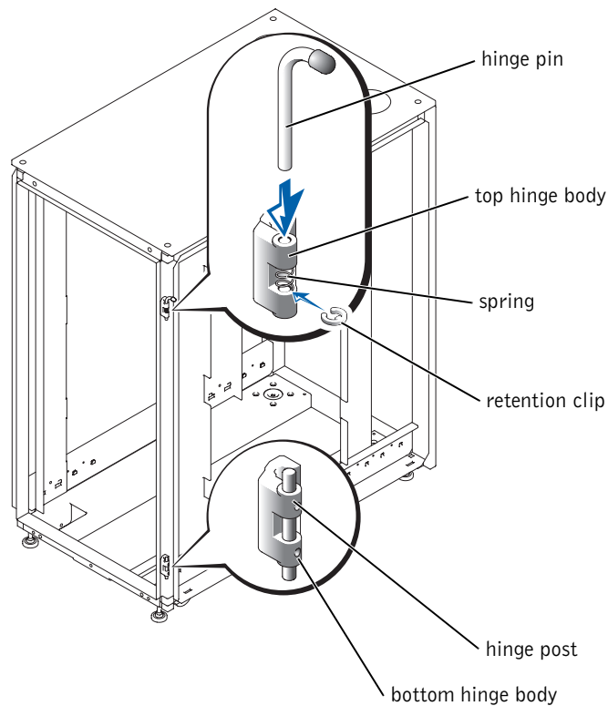
Figure 1-6. Reversing the Top and Bottom Hinges
