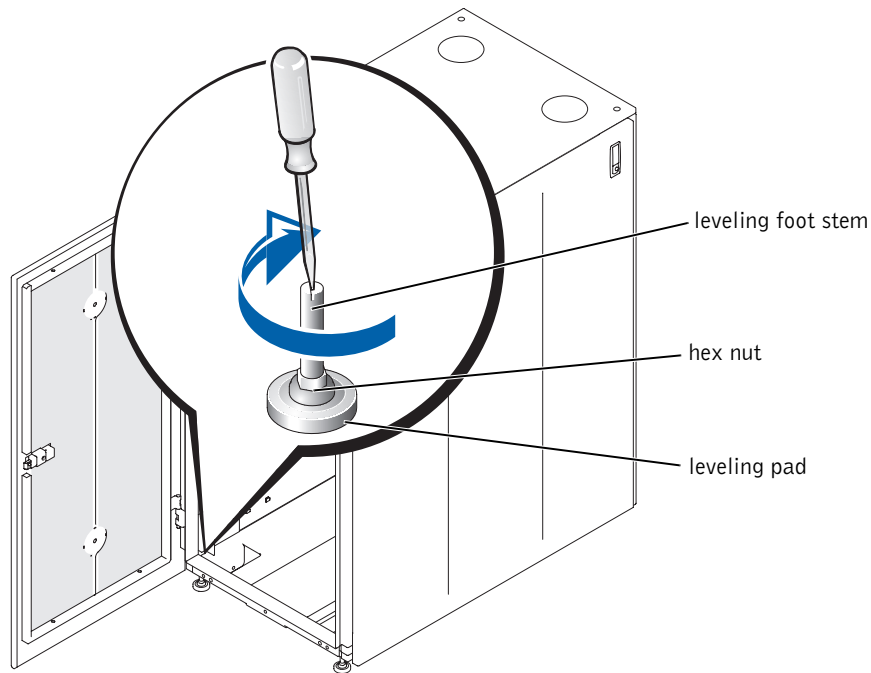
Figure 1-8. Adjusting the Leveling Feet
