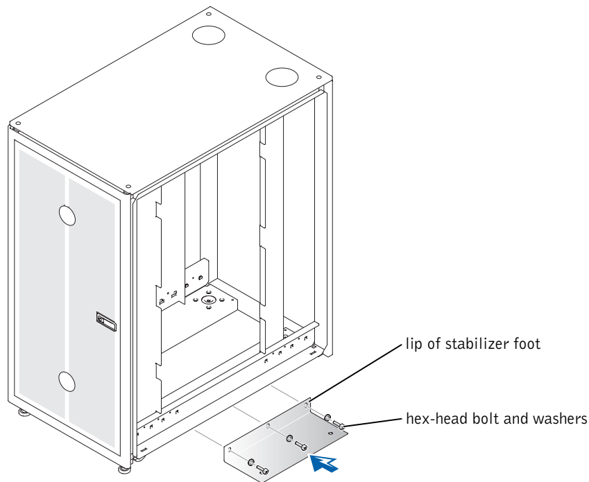
Figure 1-10. Attaching the Side Stabilizer Foot
