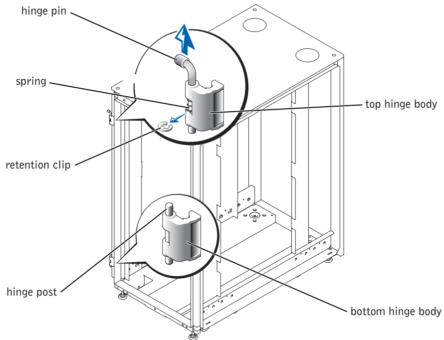
Figure 1-5. Removing the Front-Door Hinges
