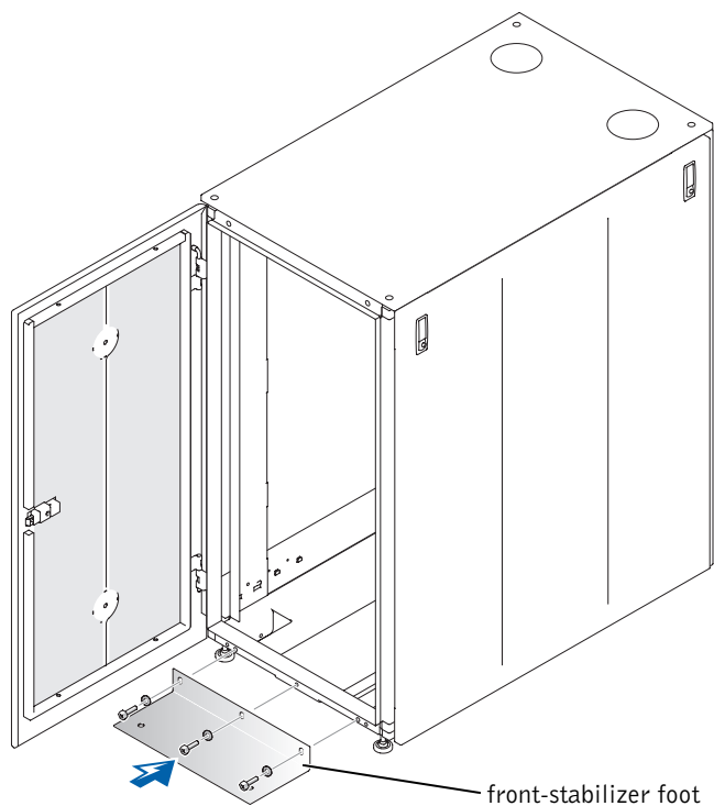
Figure 1-9. Attaching the Front Stabilizer Foot
