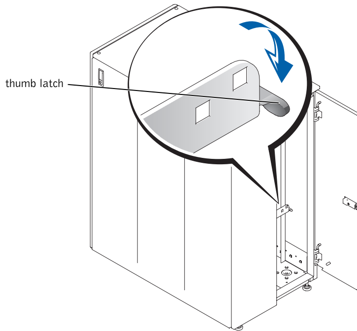
Figure 1-2. Opening the Left Back Door
