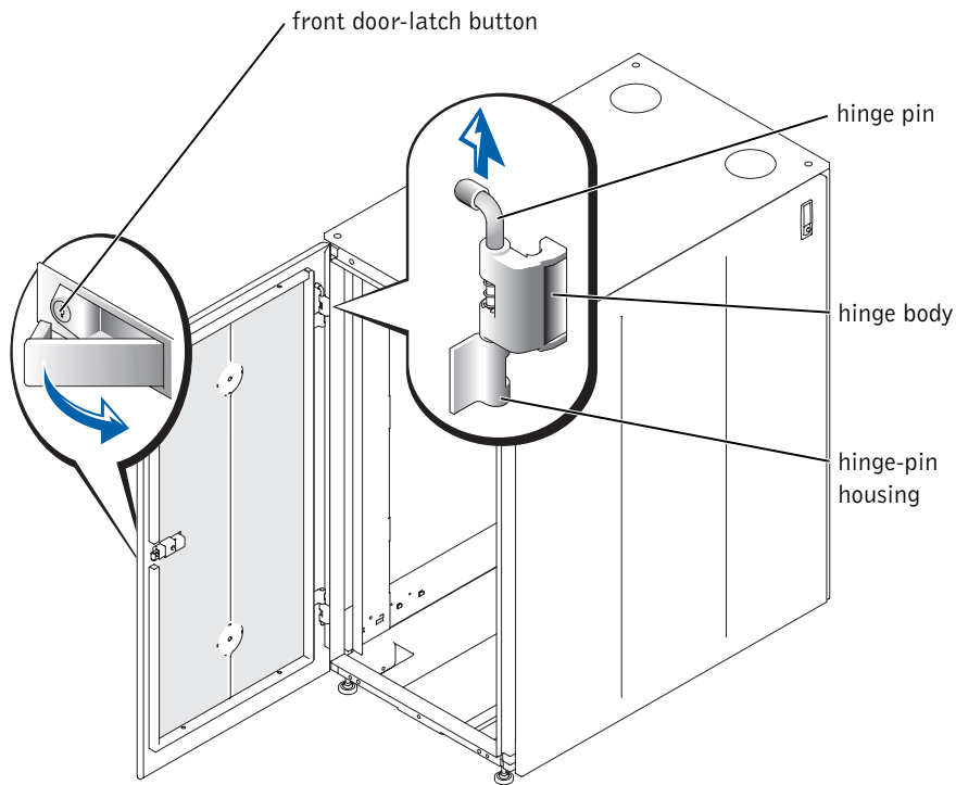
Figure 1-1. Removing the Front Door
