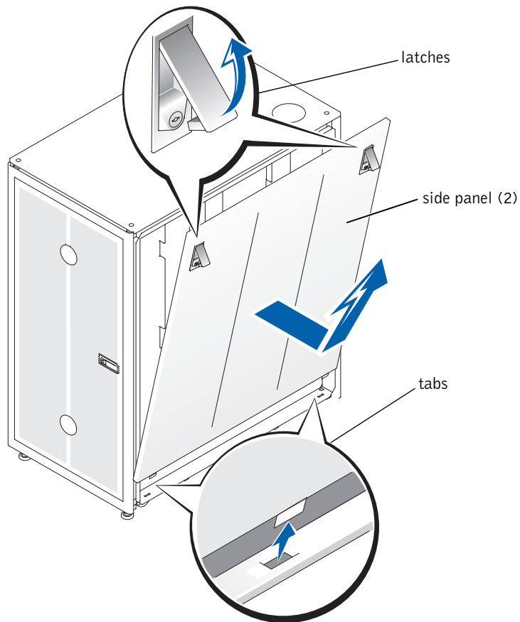
Figure 1-4. Removing a Side Panel
