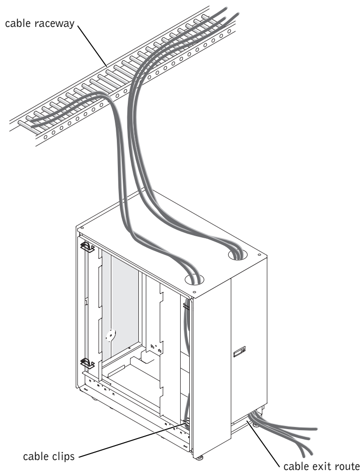
Figure 1-11. Cable-Routing Options
